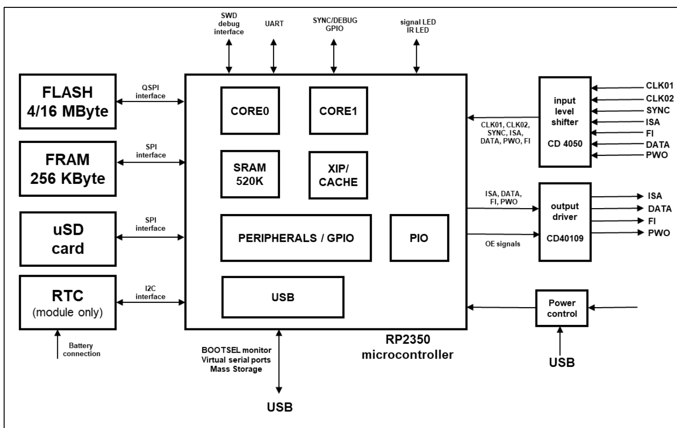
TULIP4041 BLOCK DIAGRAM
